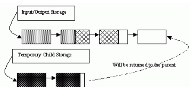
Dynamic data processing using a child storage
