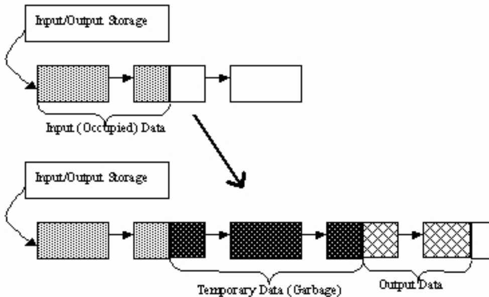
Dynamic data processing without using child storage
